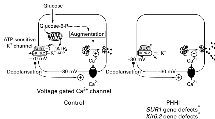
Figure 2 The sequence of events leading to the release of insulin from a pancreatic \beta cell. In brief, SUR1 and KIR6.2 constitute the ATP sensitive potassium ( K_{ATP} ) channel. These two proteins are encoded by genes located on chromosome 11p15.1. Mutations in these genes account for some cases of hyperinsulinism. The K_{ATP} channel is normally kept open maintaining a membrane resting potential of about -70 mV. When glucose enters the cell it raises the concentration ratio of ATP to ADP, which in turn causes the closure of the K_{ATP} channel. Once closed, the cell membrane becomes depolarised, allowing the influx of calcium through specific voltage gated calcium channels. This is the trigger for insulin exocytosis. Mutations have also been described in the genes for glutamate dehydrogenase (GDH) and in the glucokinase (GK) system. These defects increase the intracellular ATP to ADP ratio, thereby initiating insulin secretion. In these conditions, there is no abnormality in the potassium or calcium channel function. PHHI, persistent hyperinsulinaemic hypoglycaemia of infancy; glucose-6-P, glucose-6-phosphate. (Reproduced with permission from Shepherd et al 22 )
