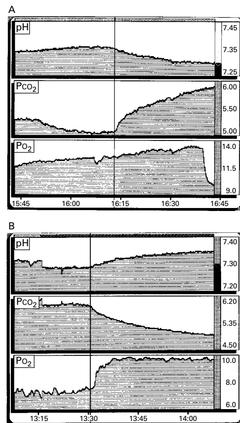
Figure 2 (A) Screen printout of multiparameter intra-arterial sensor (MPLAS) showing pH, PaCO 2 , and Pao 2 changes over a one hour period, in a 27 week gestation infant aged 9 hours. Previous chest radiograph confirmed moderate/severe respiratory distress syndrome, Fio 2 0.55. The vertical line marks t_s when there was a 3 cm H 2 O reduction in oscillatory amplitude. There is a subsequent rise in PaCO 2 (and corresponding fall in pH), but no change in the Pao 2 baseline. At the end of the study period, the Pao 2 falls sharply as Fio 2 is reduced to 0.45. (B) Screen printout of MPLAS showing pH, PaCO 2 , and Pao 2 changes over a one hour period, in the same infant 24 hours later. Previous chest radiograph confirmed improving respiratory distress syndrome, Fio 2 now 0.25. The vertical line marks t_s when there was a 3 cm H 2 O increase in oscillatory amplitude. There is a subsequent fall in PaCO 2 (and corresponding rise in pH). This is accompanied by a sharp increase in Pao 2 , completed in six minutes ( t_{\text{max}30} ), and sustained thereafter.
